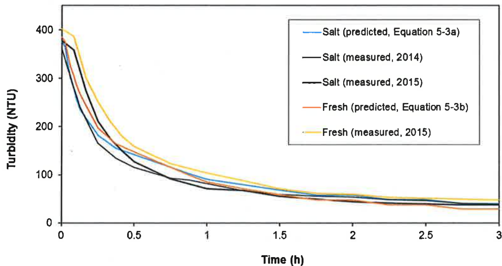
Figure 1-3: Comparison of modelled and measured turbidity. Estimates of turbidity (backscatter at 865 nm scaled to measured Normalised Turbidity Units (NTU) of salt water at t=1 second) based on Equation 5-3a and using measurements of the mass-specific backscatter of particles (Pinkerton & Gall, 2015) and effective floc densities in salt-water and fresh-water from HRW (2014).
