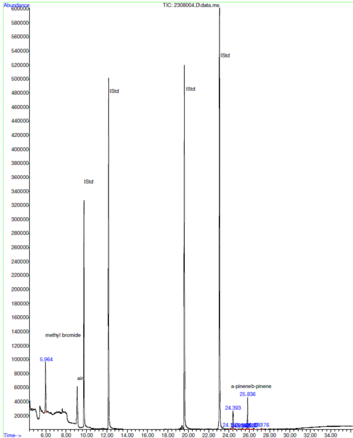
Figure 1. Total ion current chromatogram of a 10 mL injection of sample Union Taylor Ship Methyl Bromide Ventilation (222) (2228865.1), IStd = internal standard.
